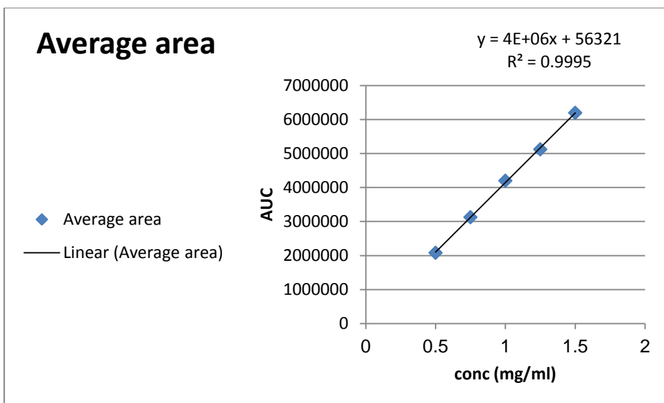
Figure 3.12. Calibration curve of atorvastatin in plasma
